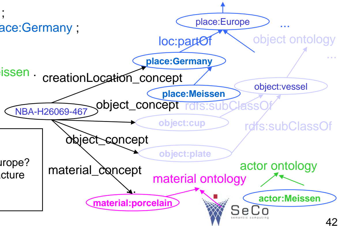
place ontology
